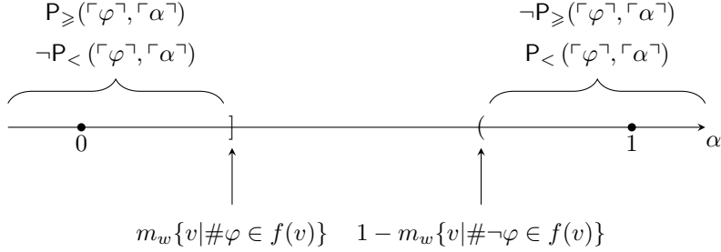
Figure 3: How \Theta(f)(w) evaluates the probability of \varphi .
