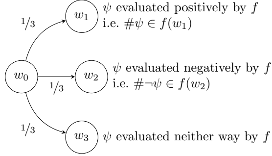
Figure 2: A fragment of a probabilistic modal structure representing the information required to evaluate P_{\geq}(\ulcorner\psi\urcorner, \ulcorner\alpha\urcorner) in \Theta(f)(w_0) .
