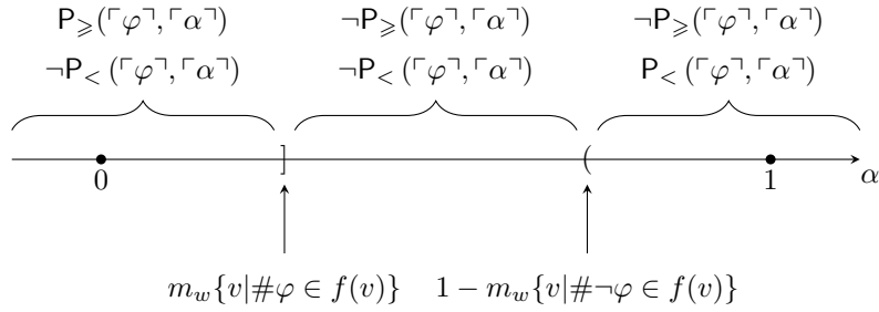
Figure 4: How \text{IndMod}_{\mathcal{M}}[w, f] evaluates the probability of \varphi
