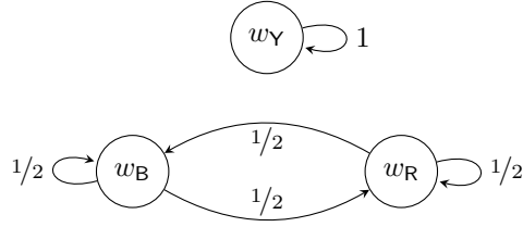
Figure 1: Example of a probabilistic modal structure.
