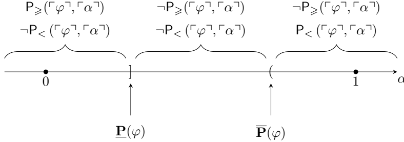
Figure 5: Definition of \underline{\mathbf{P}}(\varphi) and \overline{\mathbf{P}}(\varphi)
